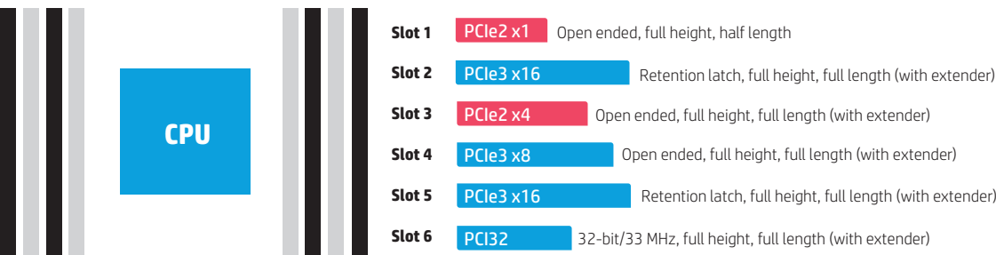
Figure 3: I/O slot layout
