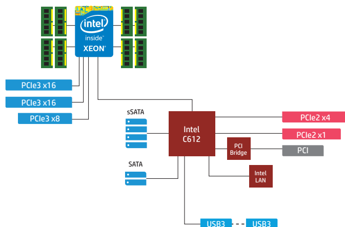
Figure 1: HP Z440 block diagram
