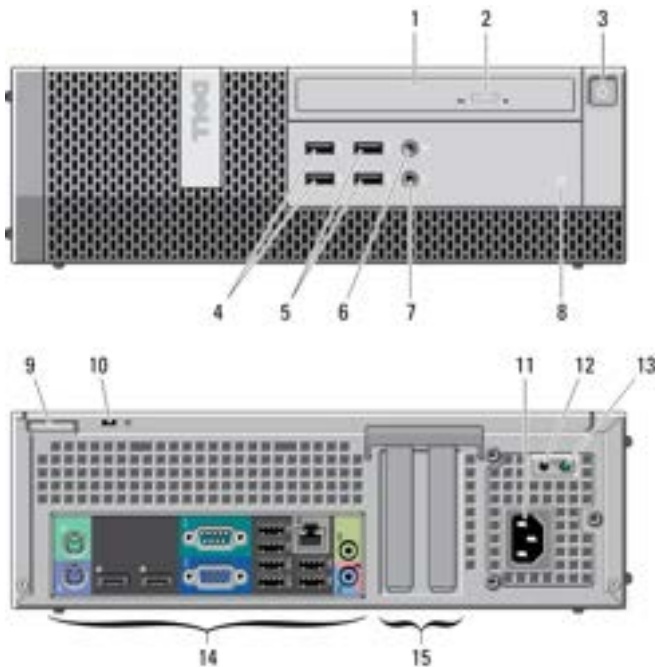
Figure 3. Back Panel view of Small Form Factor
