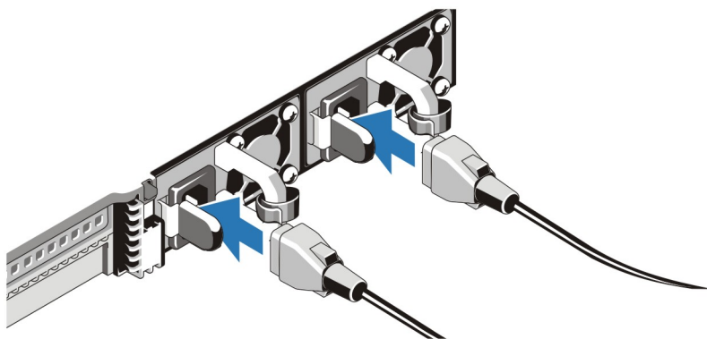
Figure 3. Connecting Power Cable(s)
