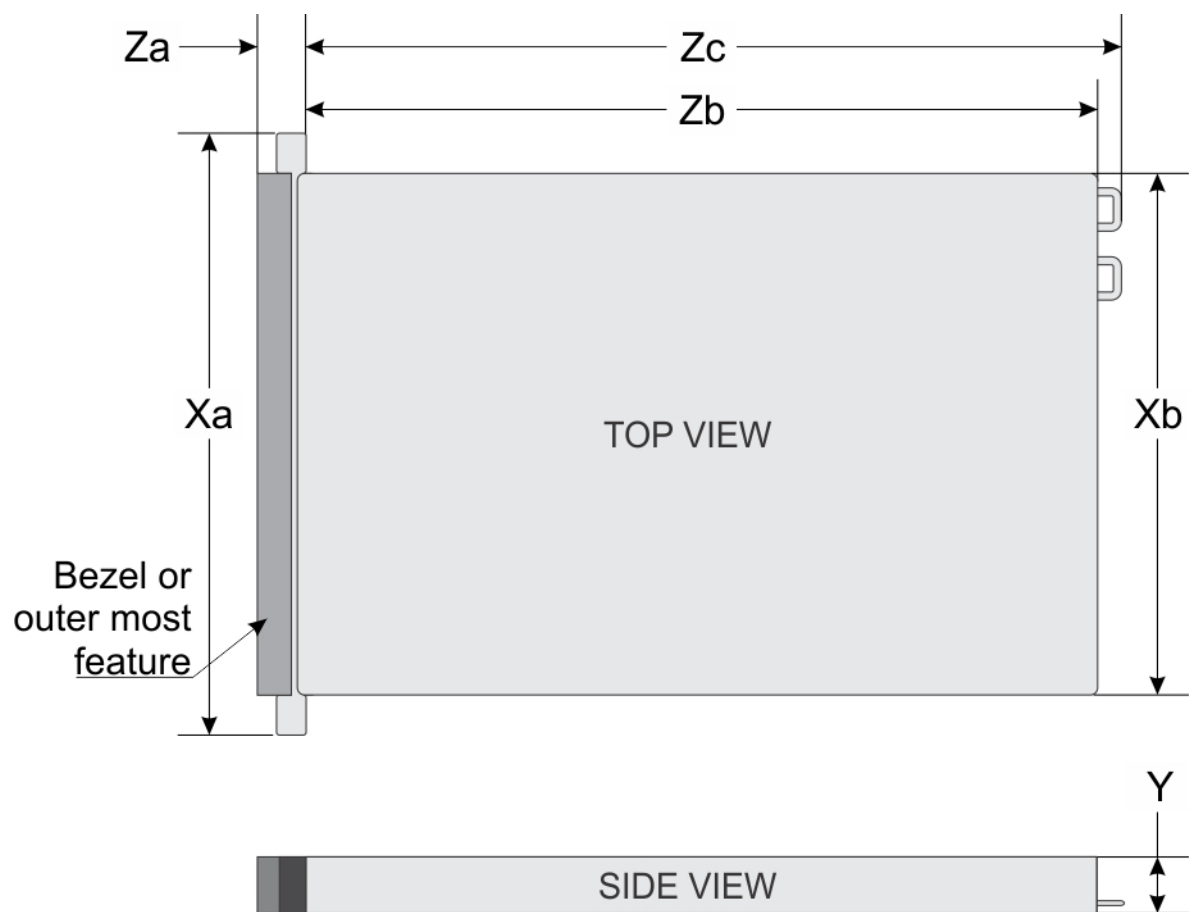
Figure 1. System dimensions
