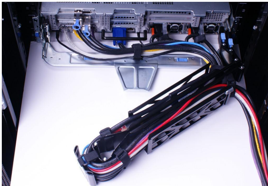
Figure 6. Right-side mounted CMA installation (CMA shown in service position)
