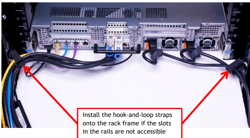
Figure 11. Cabling a system installed in static rails
