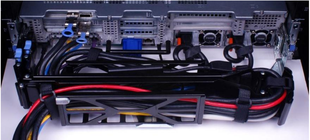
Figure 5. Left-side mounted CMA installation (preferred)
