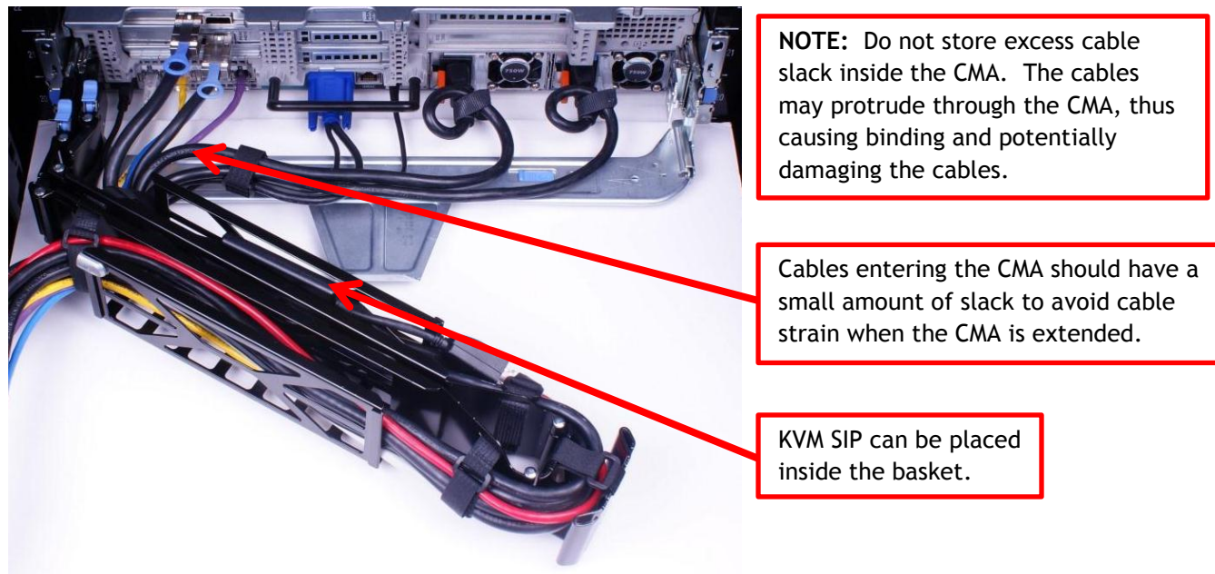
Figure 4. Routing the cables through the CMA
