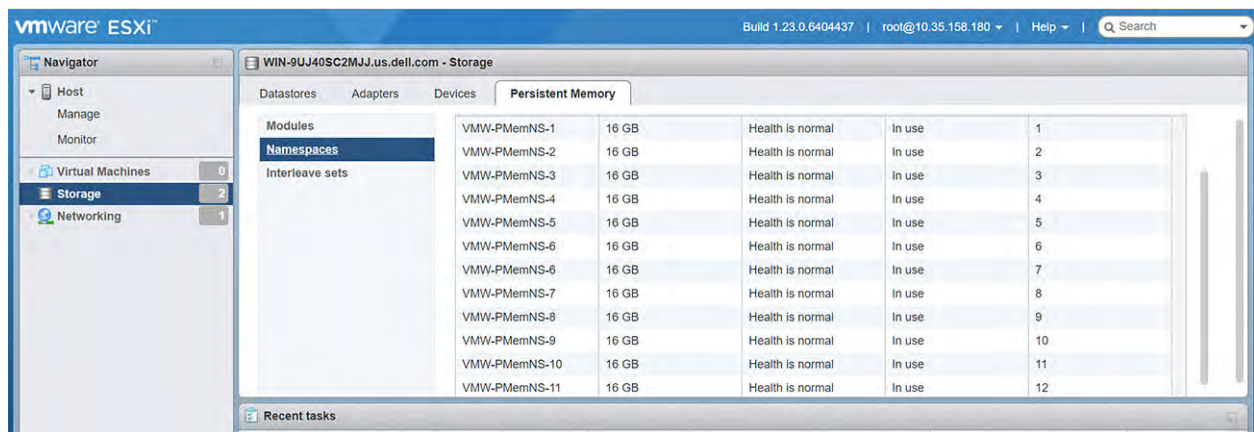
Figure 31. Namespaces
