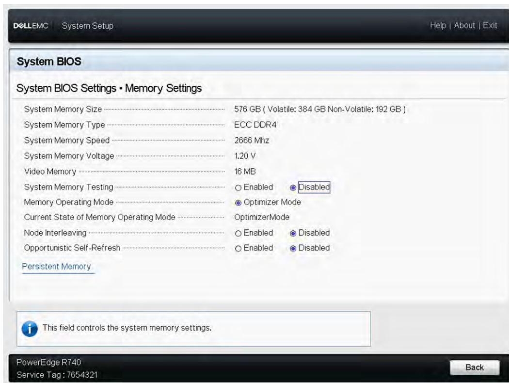
Figure 11. Memory Settings
