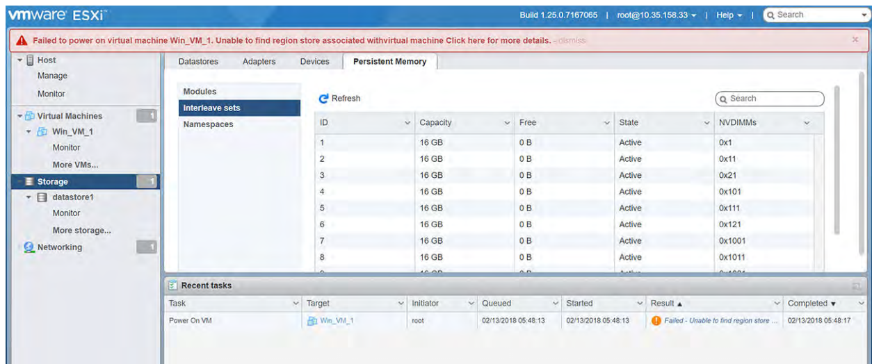
Figure 37. NVDIMM-N Errors
