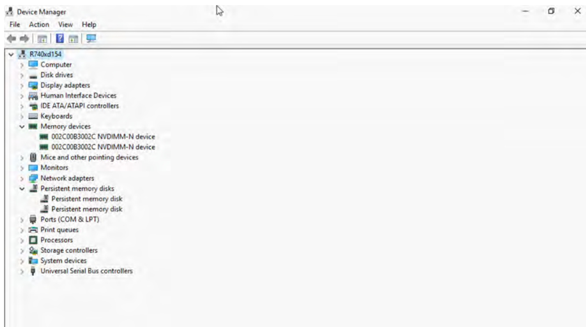
Figure 25. Device Manager
