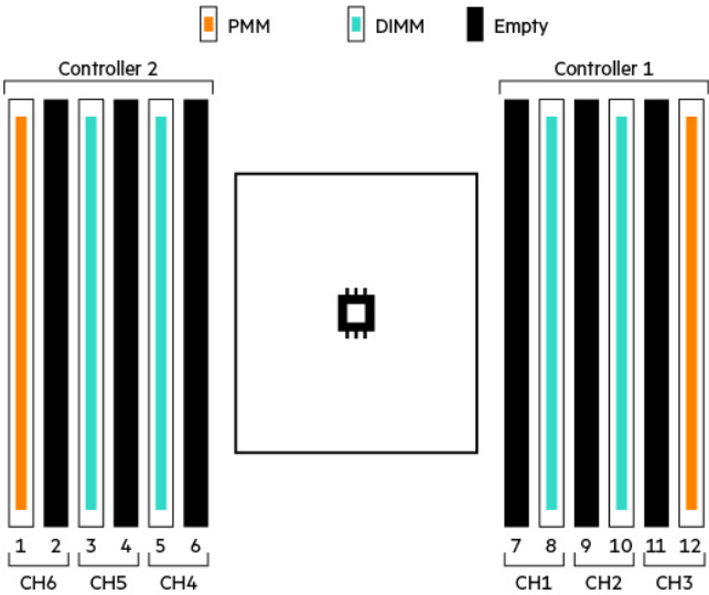
FIGURE 18. HPE Persistent Memory capacity up to 1 TB using 512 GB HPE Persistent Memory and DIMM capacity up to 512 GB using 128 GB DIMMs
