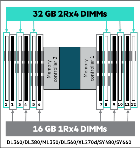
FIGURE 13. Mixing HPE SmartMemory 32 GB and 16 GB DIMMs
