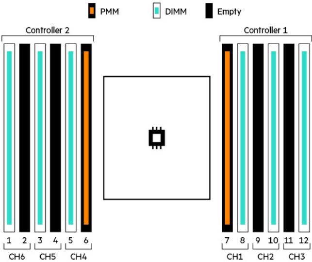
FIGURE 17. HPE Persistent Memory capacity up to 1 TB using 512 GB HPE Persistent Memory and DIMM capacity up to 768 GB using 128 GB DIMMs
