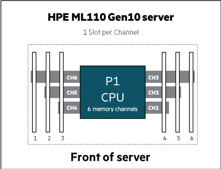
FIGURE 12. DIMM slot locations in HPE ProLiant ML110 Gen10 servers
