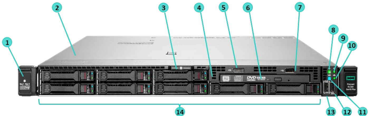
8 SFF Front View – 8 SFF + optional Universal Media Bay, optional drive, and SAS drives shown
