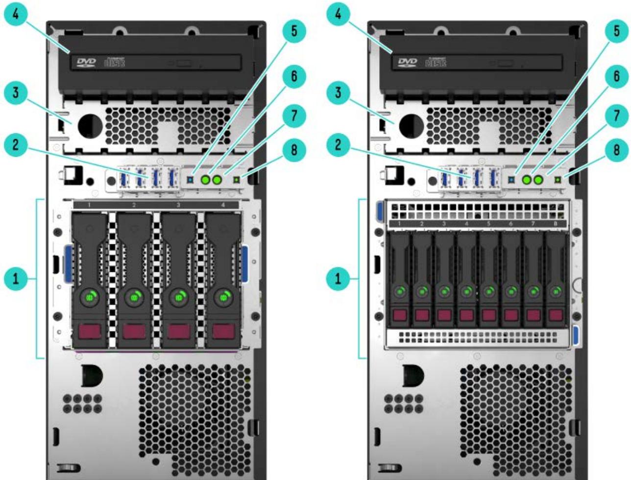
4 LFF Model
