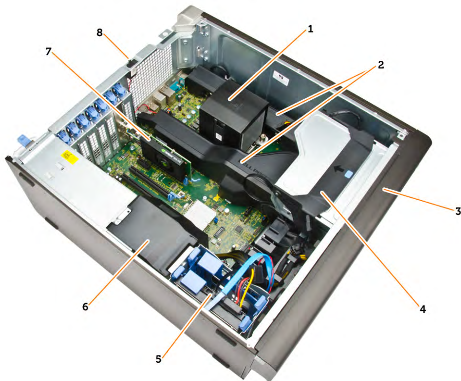
Figure 2. Inside View of T5810 Computer
