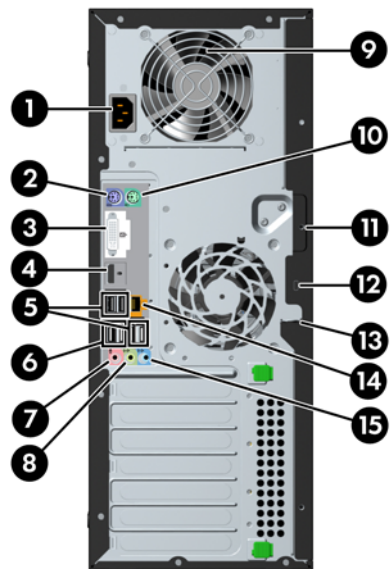
Figure 2-4 Rear panel components
