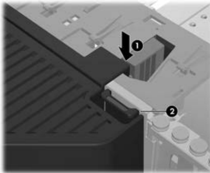
Figure 7-6 Securing the airflow guide
