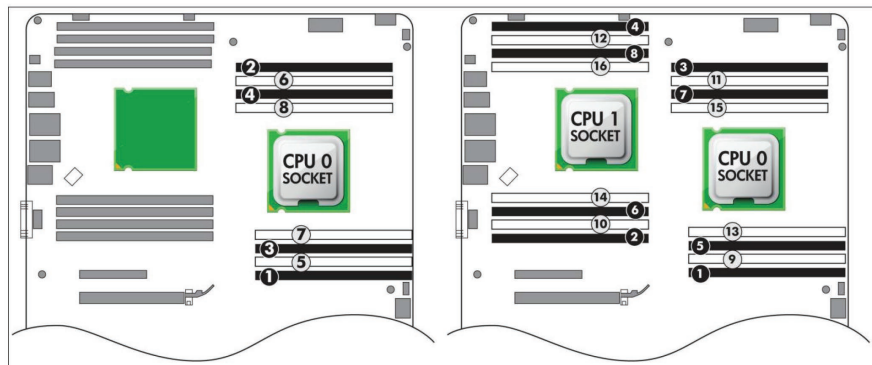
Figure 2. Load order for single and dual CPU configurations.
